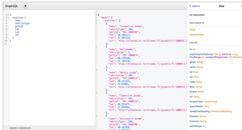
Figure 19 GraphiQL Interface — An in-browser IDE for GraphQL
